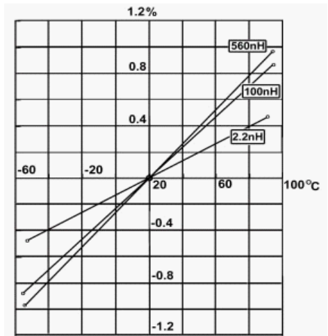
Temperature Characteristic
