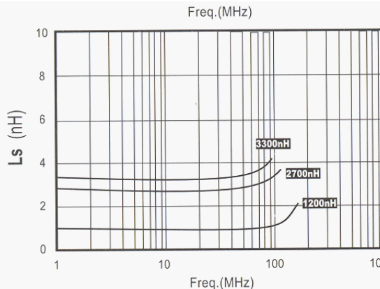
L vs Frequency
